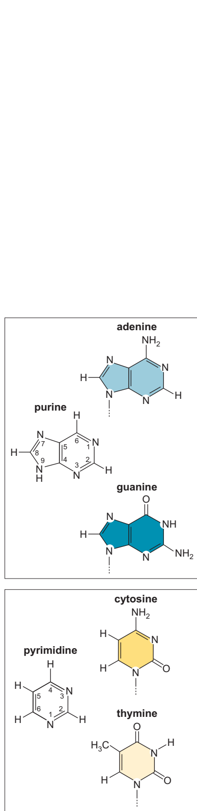
FIGURE 4-4 Purines and pyrimidines. The dotted lines indicate the sites of attachment of the bases to the sugars. For simplicity, hydrogens are omitted from the sugars and bases in subsequent figures, except where pertinent to the illustration.
