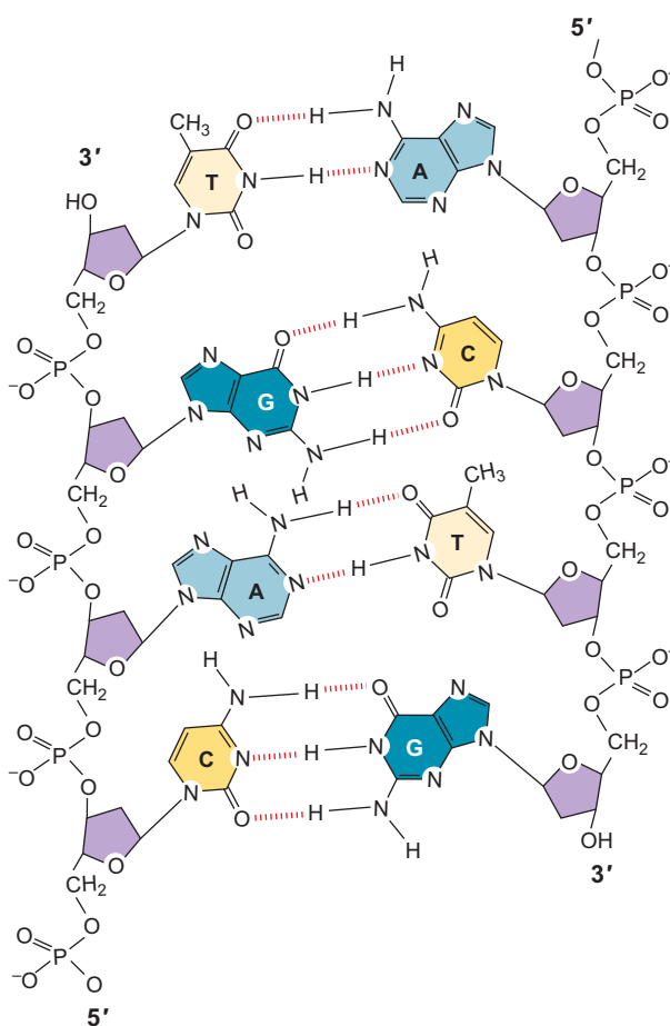
FIGURE 4-3 Detailed structure of polynucleotide polymer. The structure shows base pairing between purines (blue) and pyrimidines (yellow), and the phosphodiester linkages of the backbone. (Adapted from Dickerson R.E. 1983. Sci. Am. 249 : 94. Illustration, Irving Geis. Image from Irving Geis Collection/Howard Hughes Medical Institution. Not to be reproduced without permission.)
