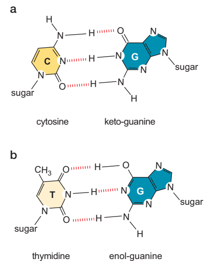
FIGURE 9-10 The tautomeric shift of guanine results in mispairing with thymidine. (a) Base pairing between the normal keto form of guanine with cytosine. (b) In the rare instance that guanine assumes the enol tautomer, it now base-pairs with thymidine instead of cytosine. Although we have illustrated the mispairing of the alternate tautomer of guanine, each of the bases can form alternate tautomers that change its base-pairing specificity.
