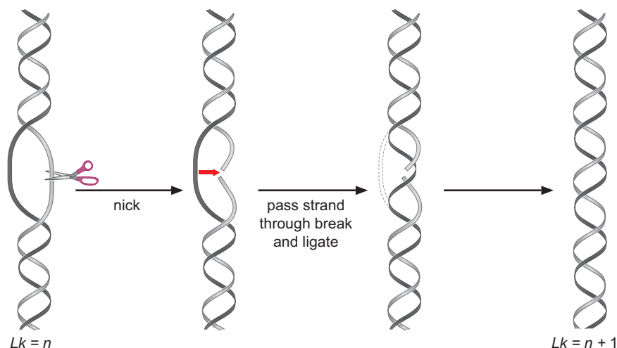
FIGURE 4-22 Schematic mechanism of action for topoisomerase I. The enzyme cuts a single strand of the DNA duplex, passes the uncut strand through the break, and then reseals the break. The process increases the linking number by +1.
